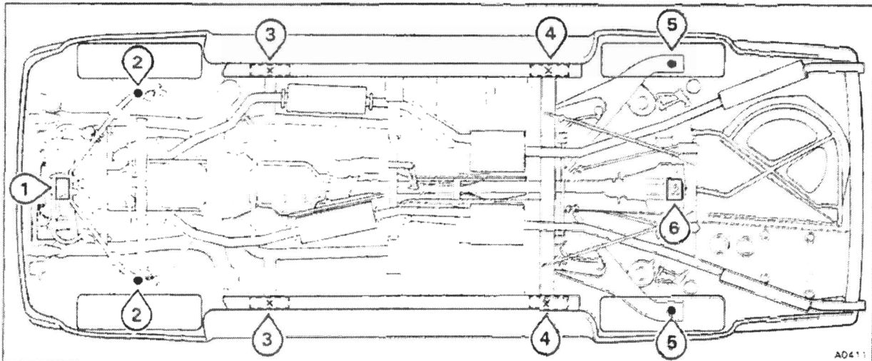
Fig. A7-1 Car jacking positions and support locations
